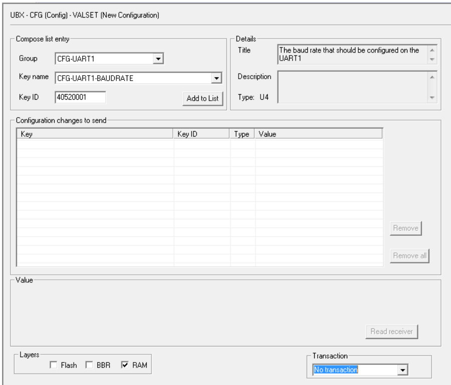
Figure 57: u-center UBX-CFG-VALSET message view
