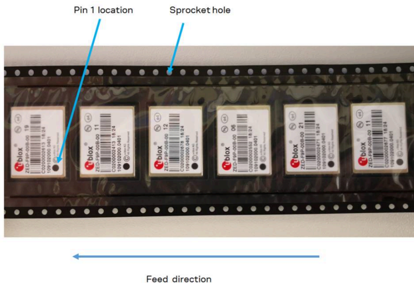
Figure 50: Orientation of ZED-F9P on the tape
